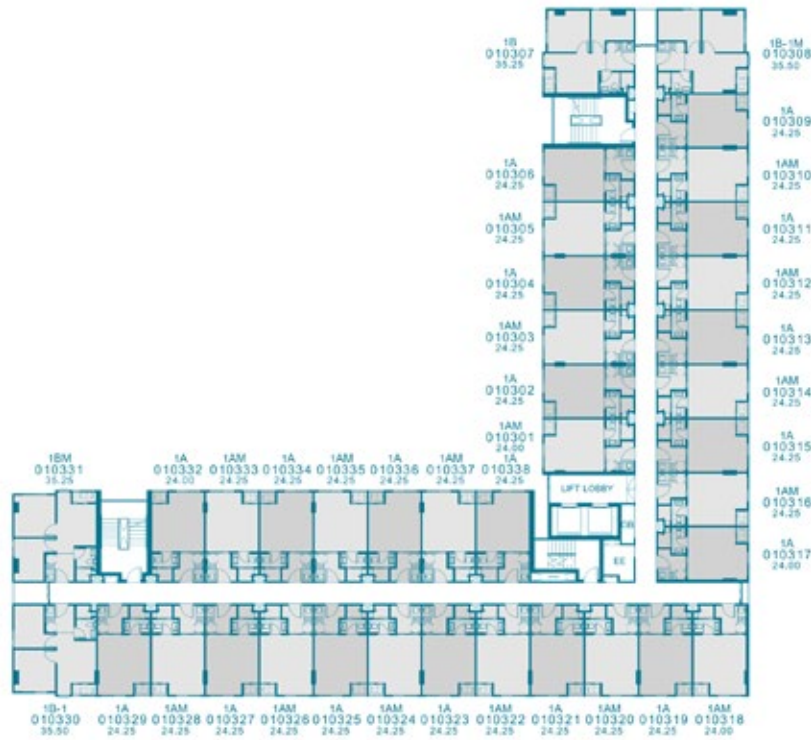
3 rd FLOOR PLAN
